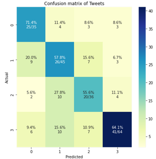
Figure 6.4 - NN (MLP). Confusion Matrix (After undersampling)
